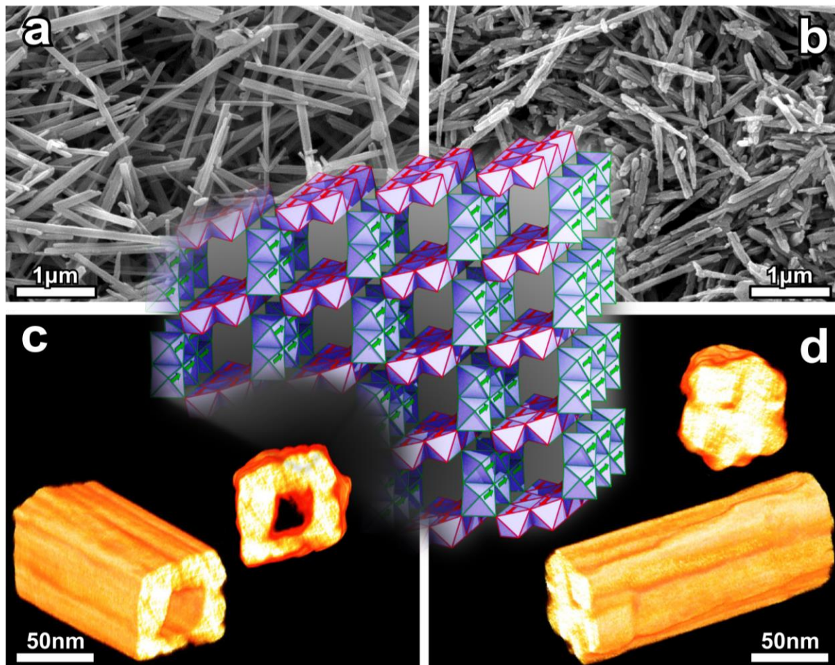
Figure 1: MnO 2 nanotubes after hydrothermal treatment, obtained from reaction mixtures pretreated in presence (a,c) and absence (b,d) of an external magnetic field ( B = 0.3 T). a and b: SEM images, c and d: Electron tomography showing the particle morphology along different viewing directions. The inset (center) illustrates the crystal structure of \alpha -MnO 2 . The differently colored octahedra symbolise opposite alignment of the magnetic moments.
