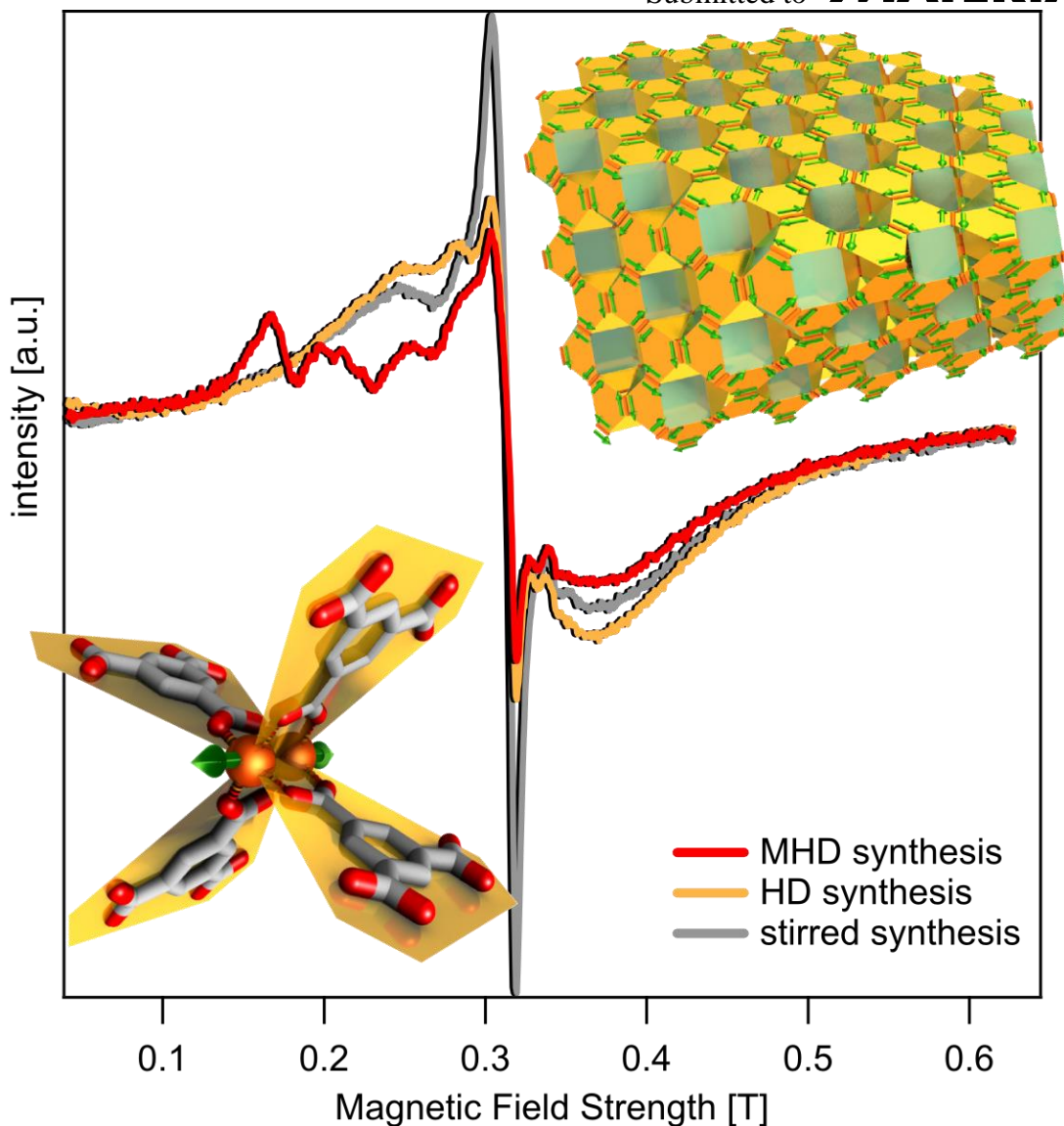
Figure 3: Room temperature EPR spectra of COK-16 for a stirred, hydrodynamic (HD) and magneto-hydrodynamic (MHD) synthesis using a static magnetic field of 0.3 T. Measurements at 140 K are provided in the supplementary material (Figure S1). The inset on the left shows a Cu paddle wheel, the basic building block of the structure. The one on the right provides a general view of the COK-16 structure, where the Cu-pairs are arranged in a Kagomé lattice [32] in the 111 planes. Green arrows illustrate the alignment of the magnetic moments.
